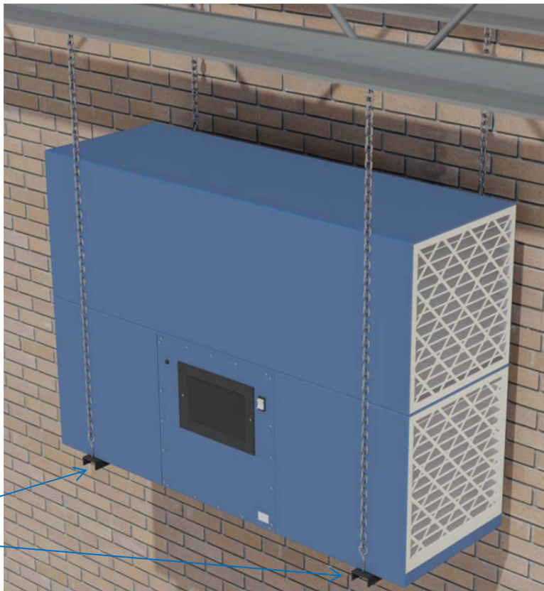
Strut Channel Installed to Ceiling Truss
